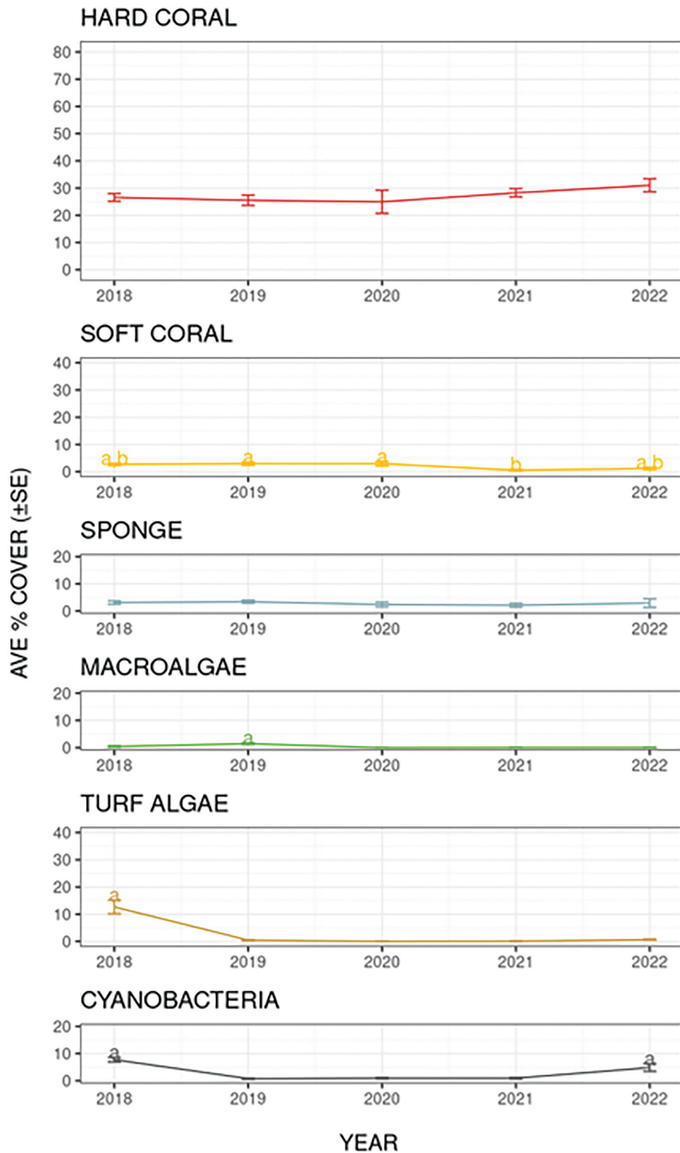
Figure A2.13. Comparison of cover of benthic components ( \pm standard error) across Station 2B, North Atoll. Years marked with different letters are significantly different.
