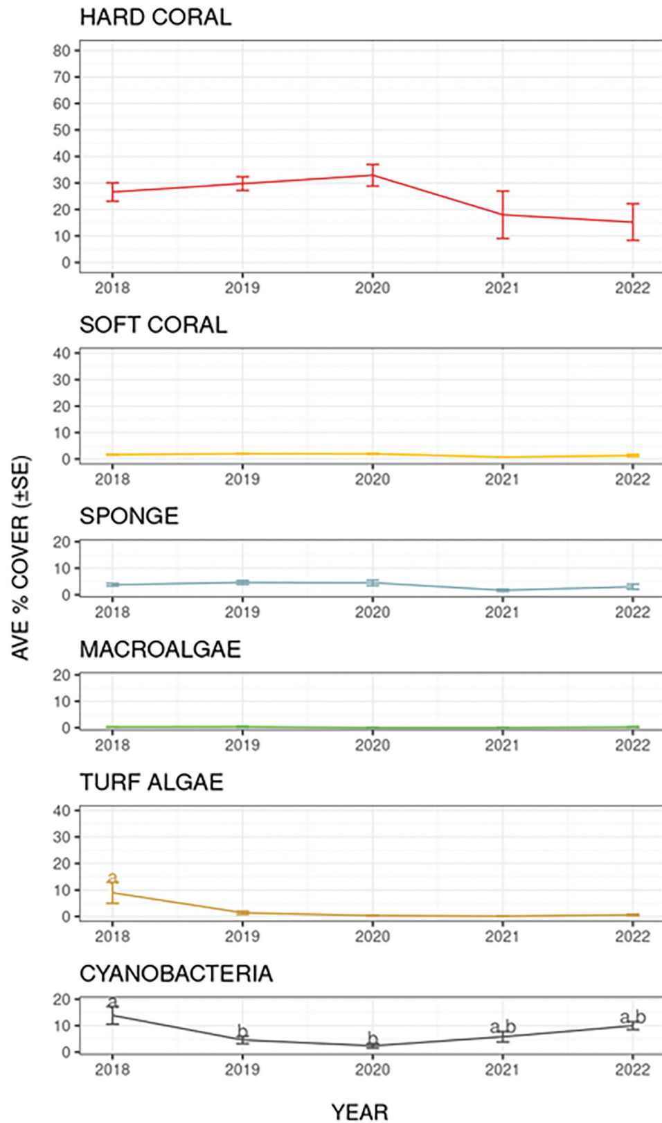
Figure A2.15. Comparison of cover of benthic components ( \pm standard error) across Station 3B, South Atoll. Years marked with different letters are significantly different.
