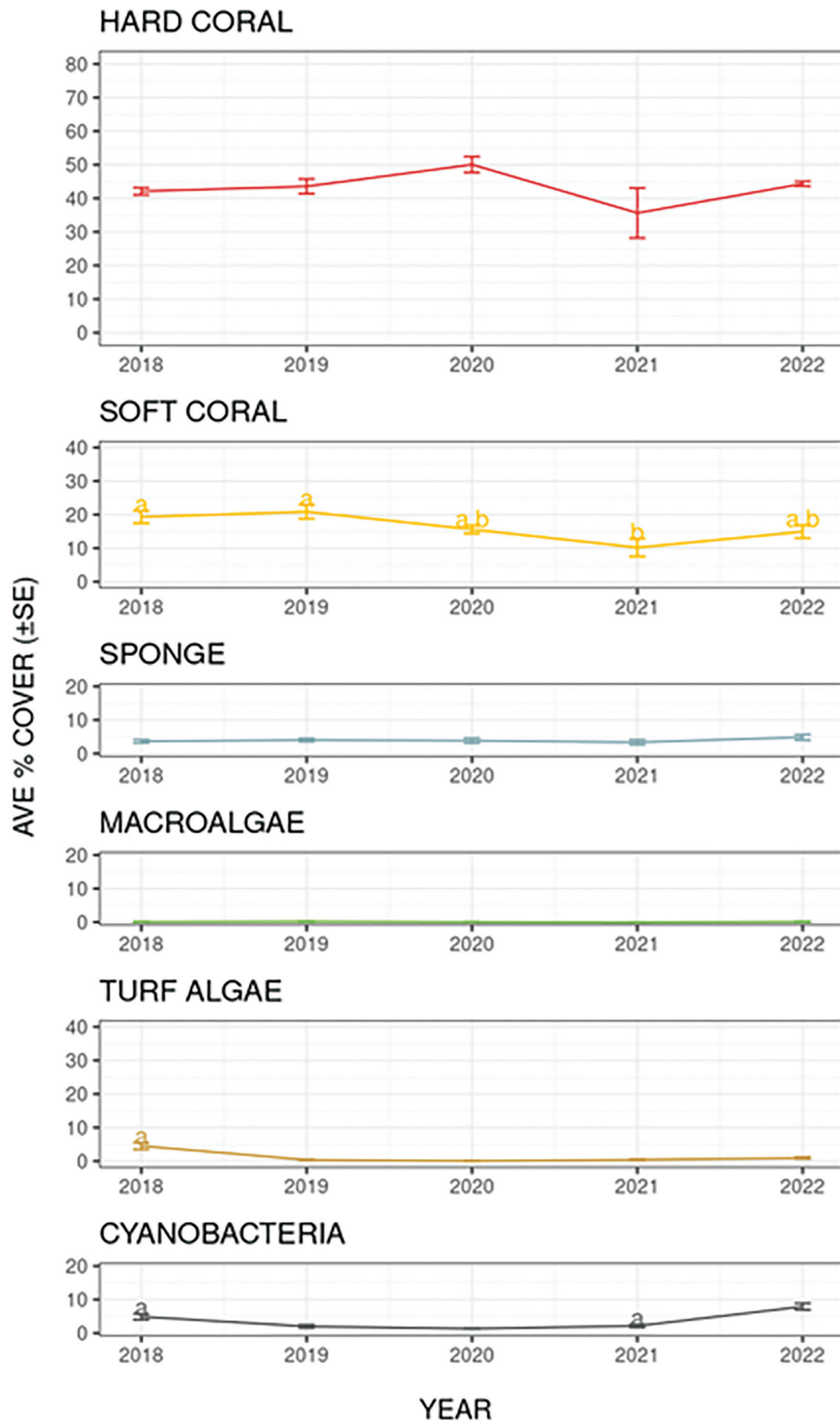
Figure A2.11. Comparison of cover of benthic components ( \pm standard error) across Station 1B, North Atoll. Years marked with different letters are significantly different.
