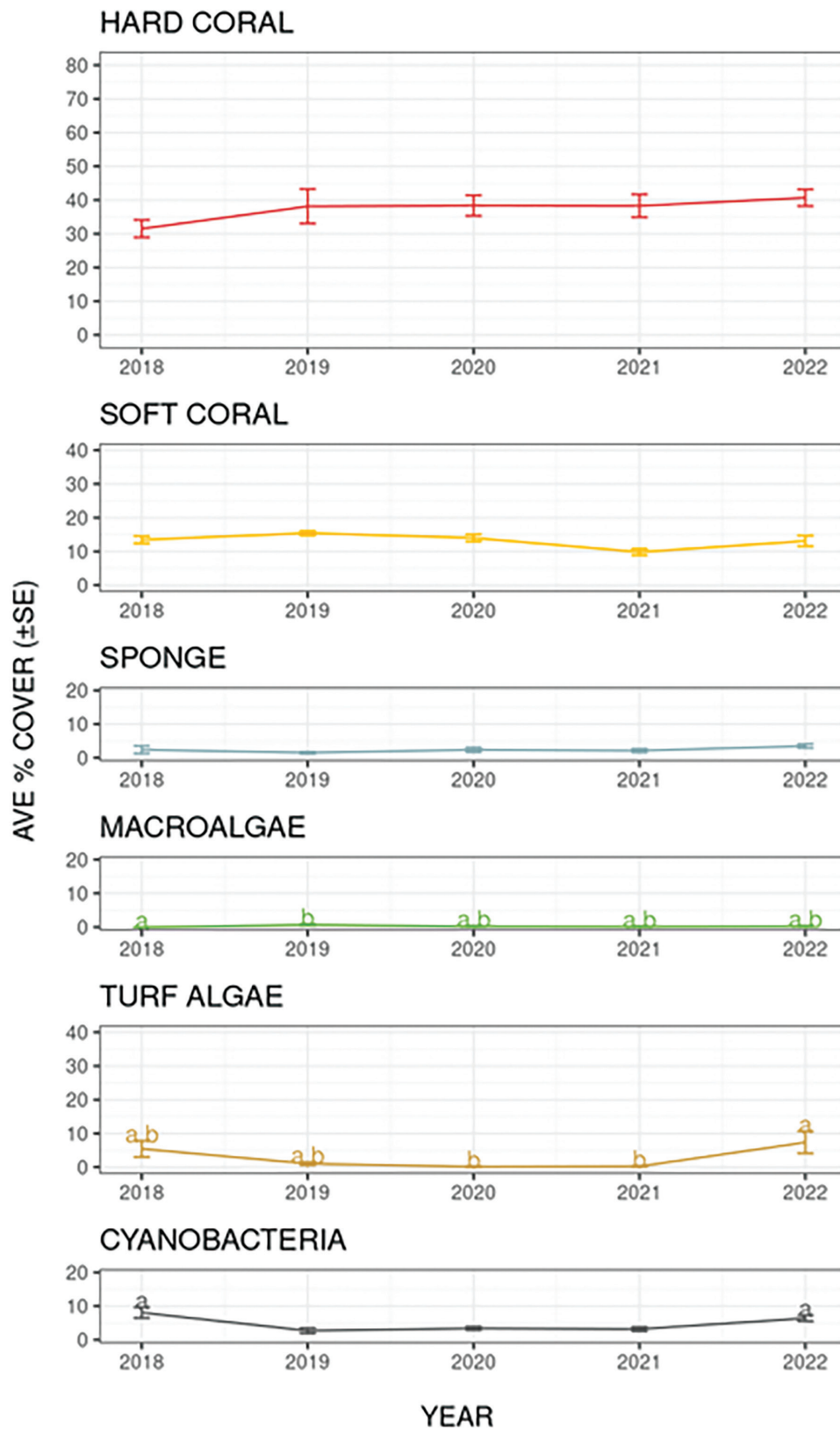
Figure A2.19. Comparison of cover of benthic components ( \pm standard error) across Jessie Beazley B. Years marked with different letters are significantly different.
