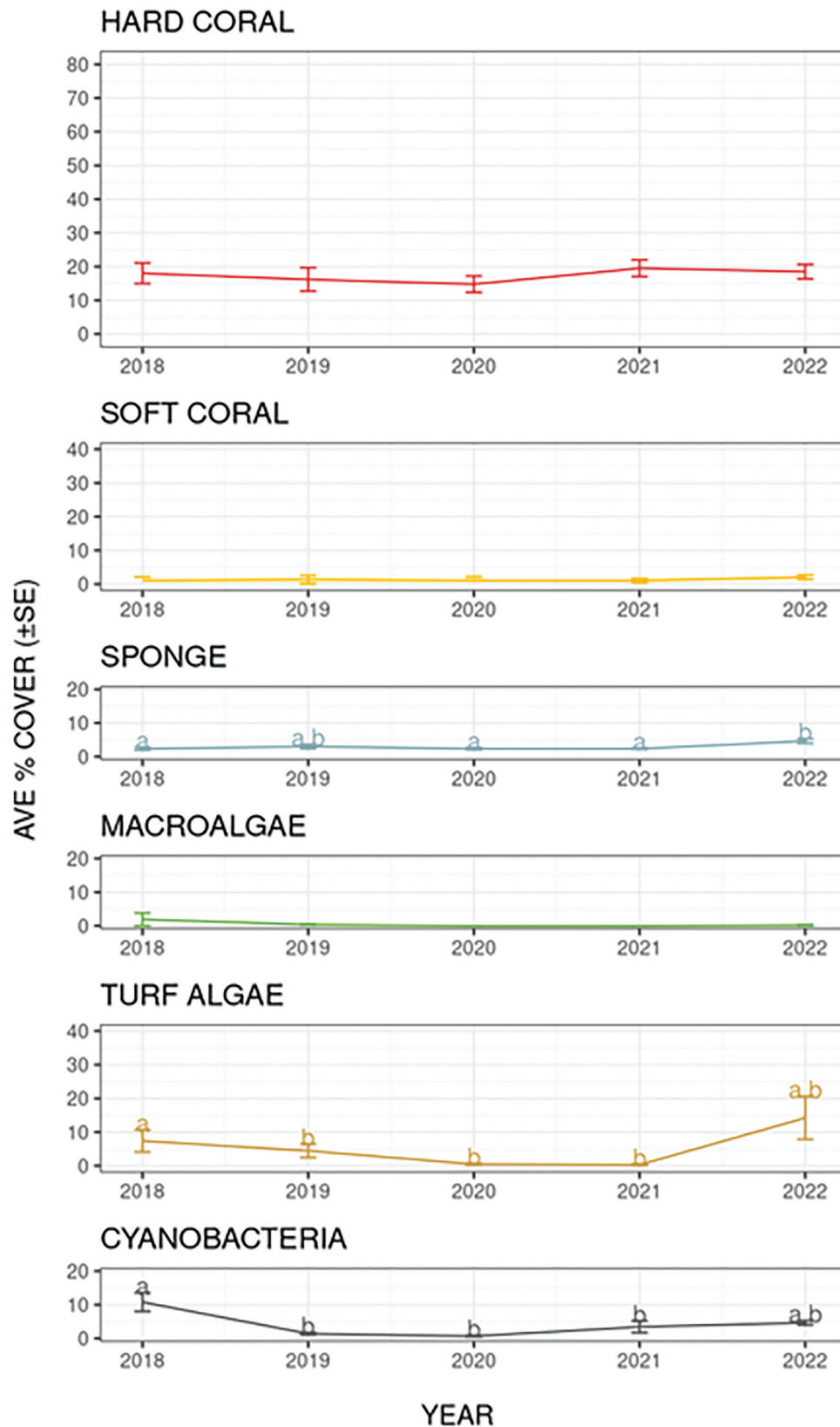
Figure A2.16. Comparison of cover of benthic components ( \pm standard error) across Station 4A, South Atoll. Years marked with different letters are significantly different.
