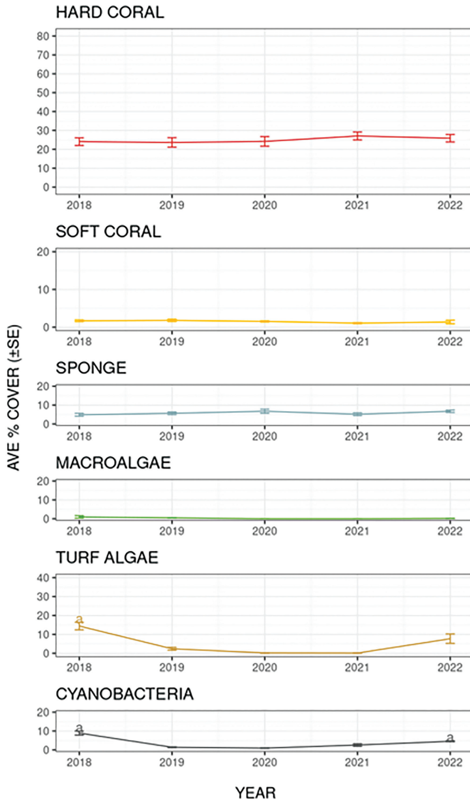
Figure A2.9. Comparison of cover of benthic components ( \pm standard error) across Site 4, South Atoll. Years marked with different letters are significantly different.
