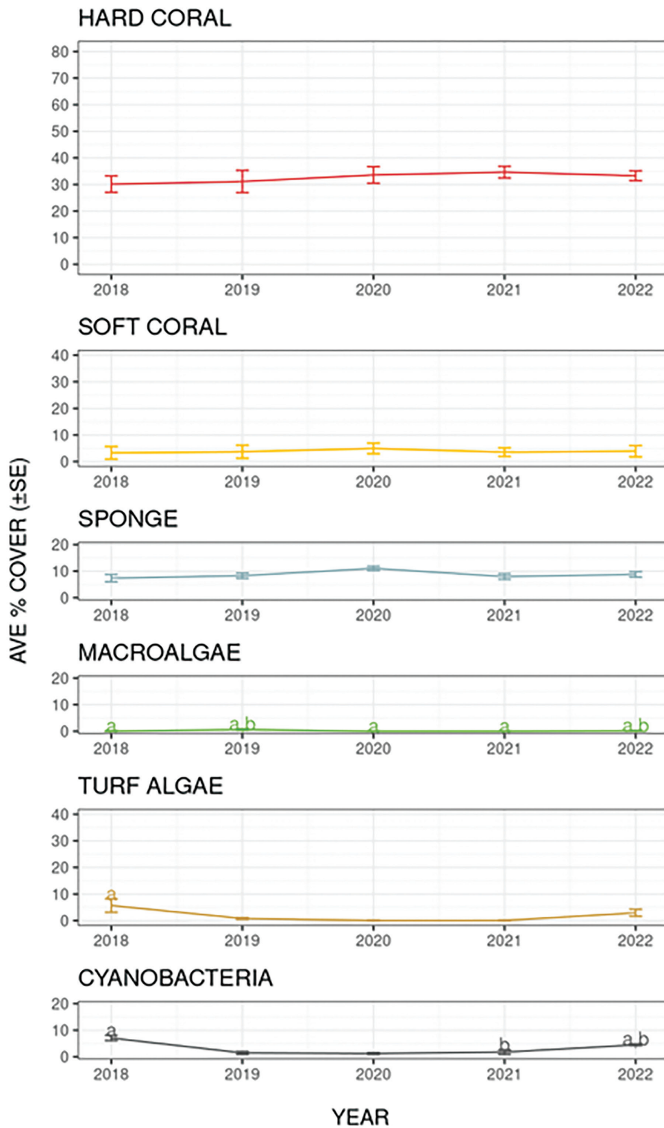
Figure A2.17. Comparison of cover of benthic components ( \pm standard error) across Station 4B, South Atoll. Years marked with different letters are significantly different.
