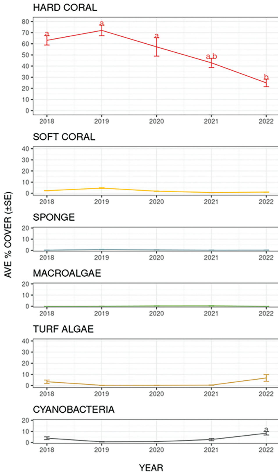
Figure A2.18. Comparison of cover of benthic components ( \pm standard error) across Jessie Beazley A. Years marked with different letters are significantly different.
