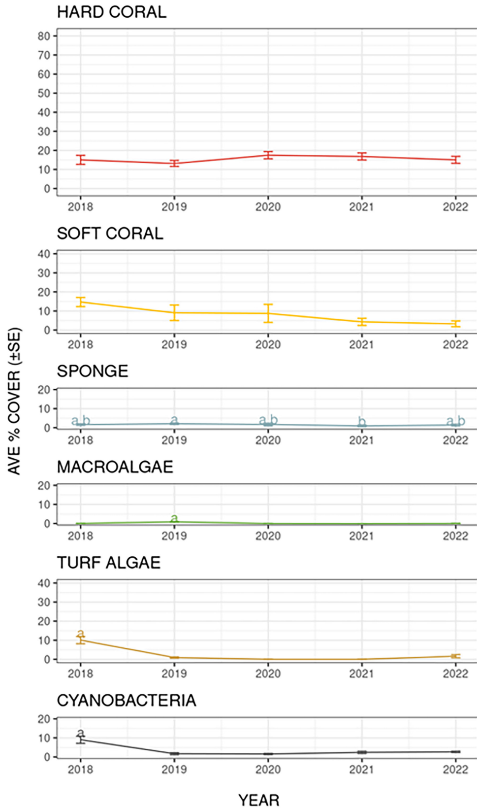
Figure A2.12. Comparison of cover of benthic components ( \pm standard error) across Station 2A, North Atoll. Years marked with different letters are significantly different.
