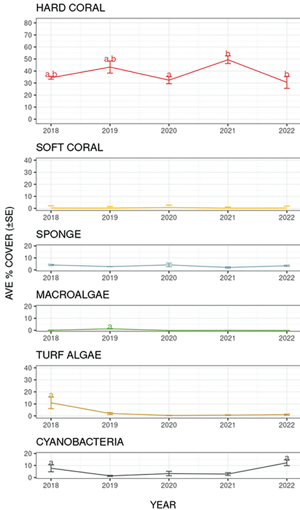
Figure A2.14. Comparison of cover of benthic components ( \pm standard error) across Station 3A, South Atoll. Years marked with different letters are significantly different.
