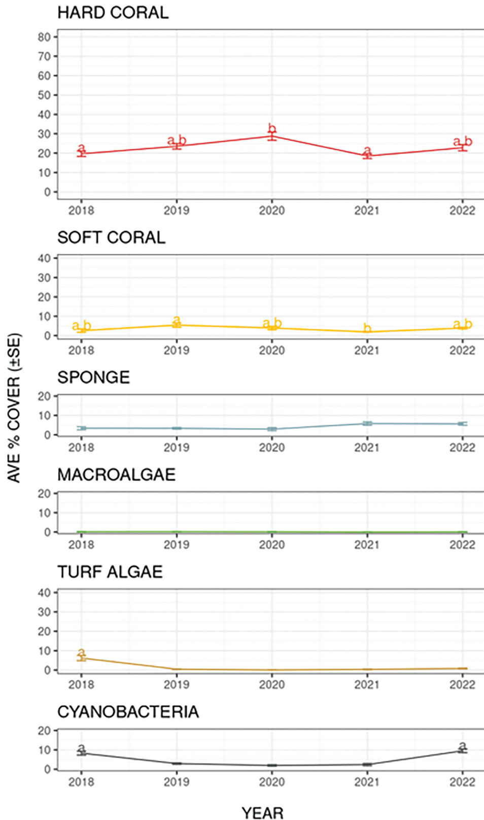
Figure A2.10. Comparison of cover of benthic components ( \pm standard error) across Station 1A, North Atoll. Years marked with different letters are significantly different.
